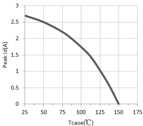
Figure 11. Current Derating
