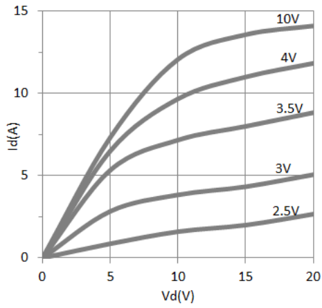
Figure 1. Typical Output Characteristics T_j=25^\circ\text{C}
