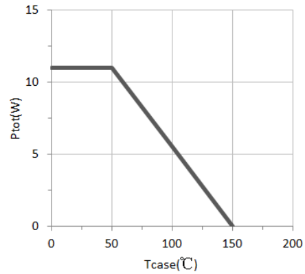
Figure 10. Power Dissipation
